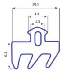
AP 05 5MM E TYPE
