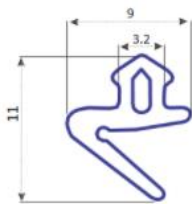
AP 06 SASH SEAL
