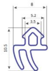
AP 09 K TYPE
