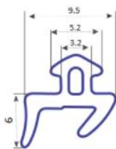
AP 07 K TYPE
