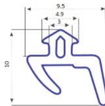
AP 08 K TYPE
